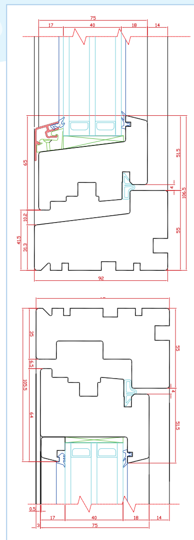
Cross-section of the SW 11 window
